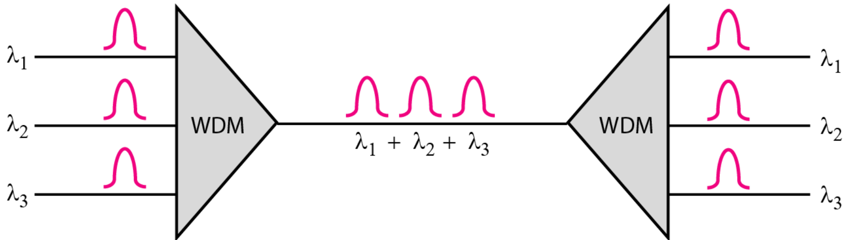
Figure 6.10 Wavelength-division multiplexing
